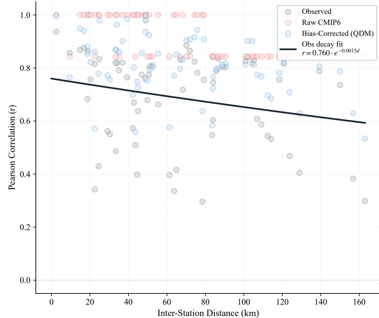
(a) Distance-Decay Relationship (Physical consistency test: r decreases with distance)
