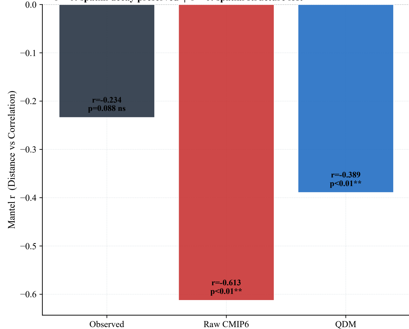
(b) Mantel Test Results r < 0 : spatial decay preserved | r > 0 : spatial structure lost
